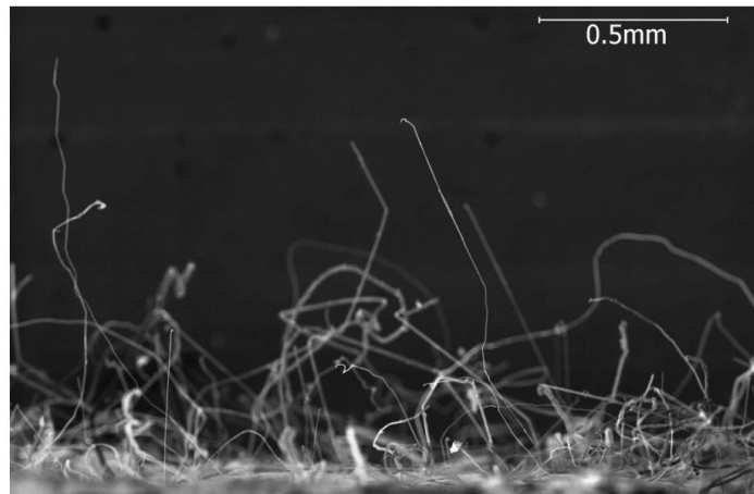
Very High Density of Zinc Whiskers
